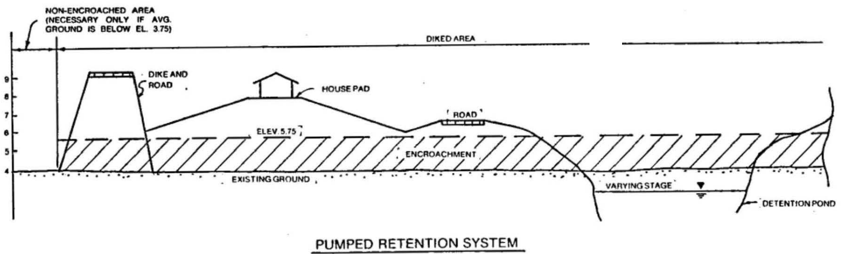
Figure 41-2 TYPICAL DEVELOPMENT SCHEMES
